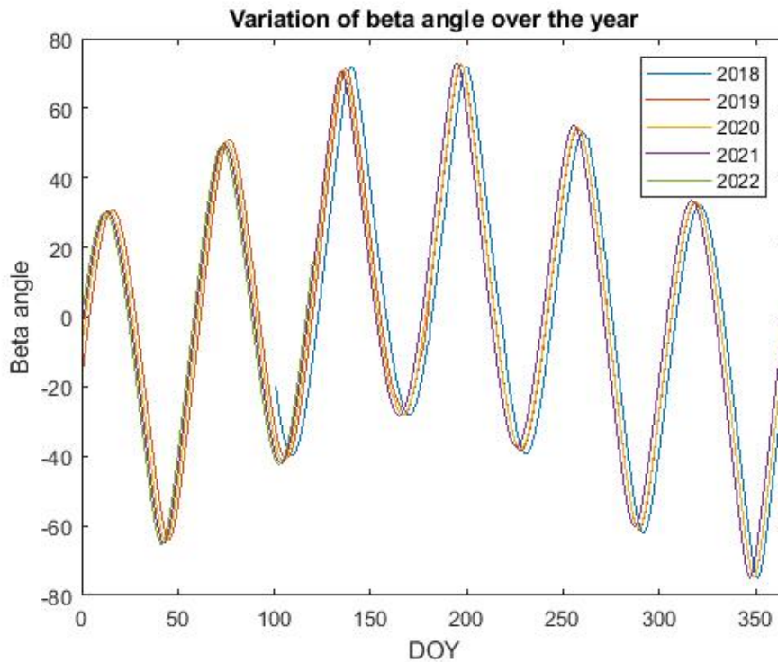
Figure 2: Beta angle vs DOY. Max beta angle is shifted back 2-3 days/year for actual beta angle. Predicted beta angle is shifted back 1 day/year.
