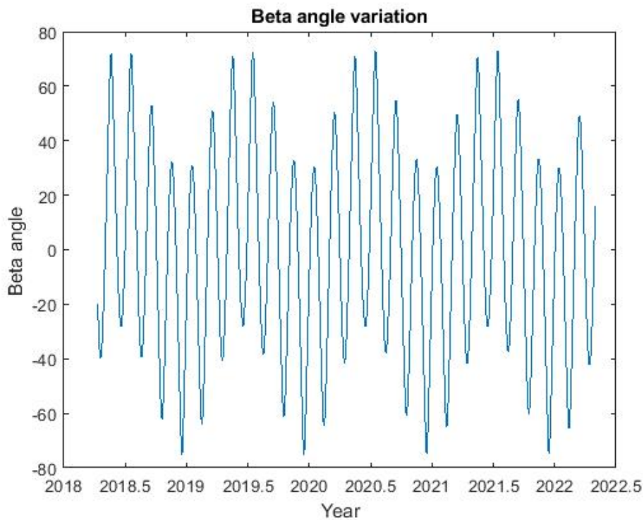
Figure 1: Beta angle. Fast variation is due to precession of ISS orbit, slow variation is seasonal.
